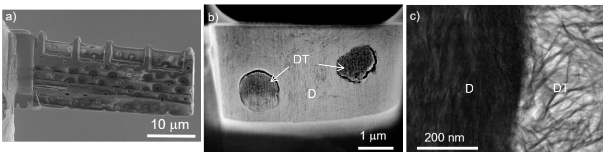
Figure 12: Sample preparation of rodent dentine (D) by a combination of UM, FIB and NM. (a) SEM image of the lamellae, (b) HAADF-STEM image and (c) BF-STEM image.
