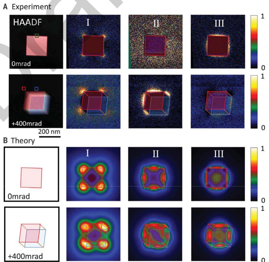
Figure 2 : 2D phonon mapping at different tilt angles. (A) (Left) Experimental HAADF images and (right) fitted maps of the main experimental SPhP modes (I, II, and III) for two tilt configurations (0 and 400 mrad) (materials and methods). The face in contact with the substrate is highlighted with a blue square. (B) Same for simulations of a cube in vacuum.
