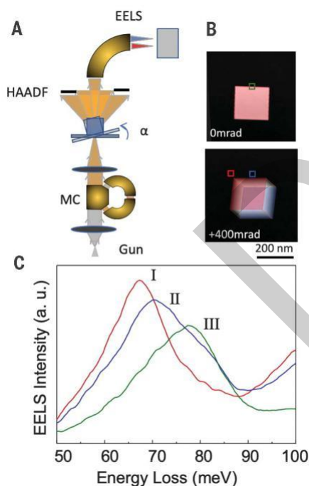
Figure 1 : Tomographic SPhP EELS experiments.
